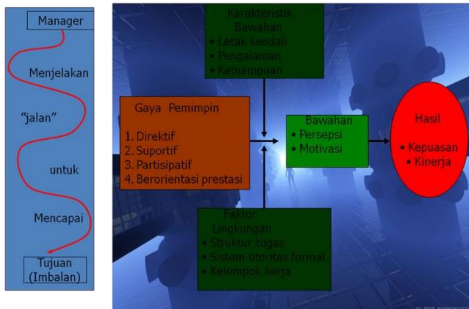
Gambar 1.3 Model Teori Jalur Tujuan (Path-Goal Theory)
